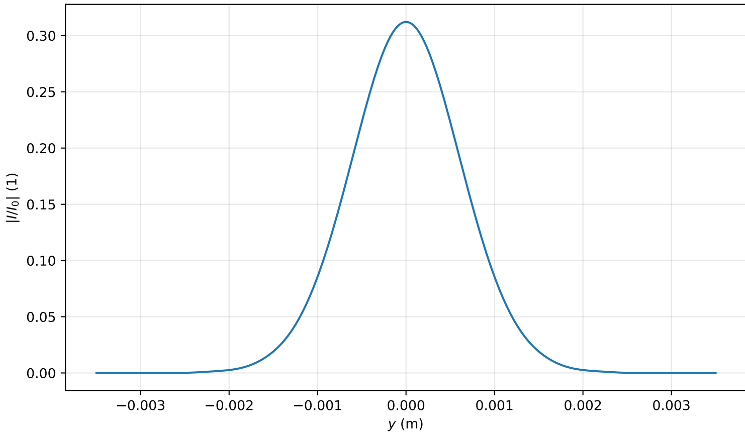
Intensity profile I(x = 0, y, z = 3.423)/I_0 , P_{in}=0.2P_{cr} , artificial time
